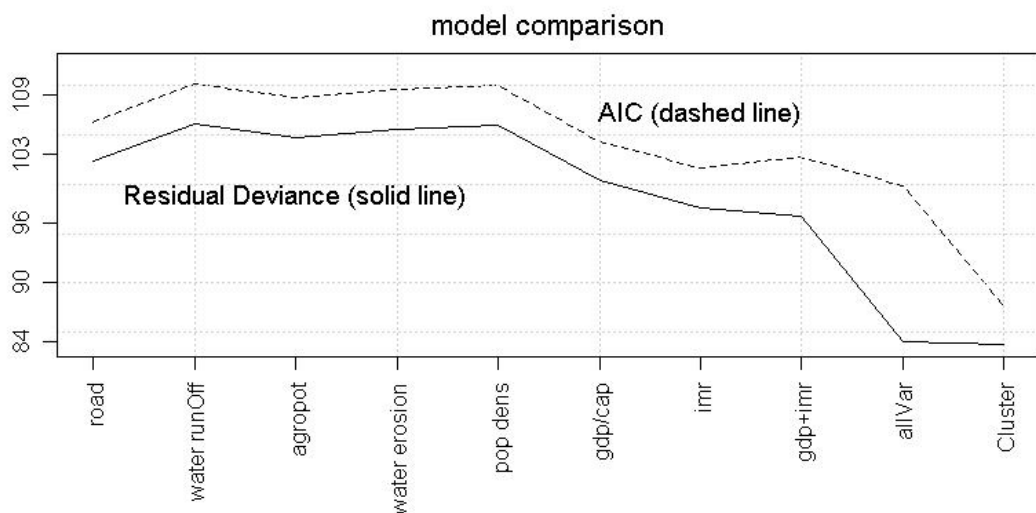
Fig. 2 AIC and residual deviance for the models. AIC and residual deviance for comparing the models of the monovariate logit fit for each of the seven drylands indicators, the multivariate logit fits for income and IMR, all drylands indicators, and the country cluster index as the explanatory variable. Smaller values denote better fits. See Table 1 for full indicator names
