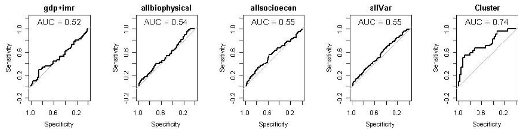
Fig. 3 ROC for comparing the models of the multivariate logit fits for income and IMR, biophysical indicators, socio-economic indicators, all drylands indicators, and the country cluster index as the explanatory variable (from left to the right)
