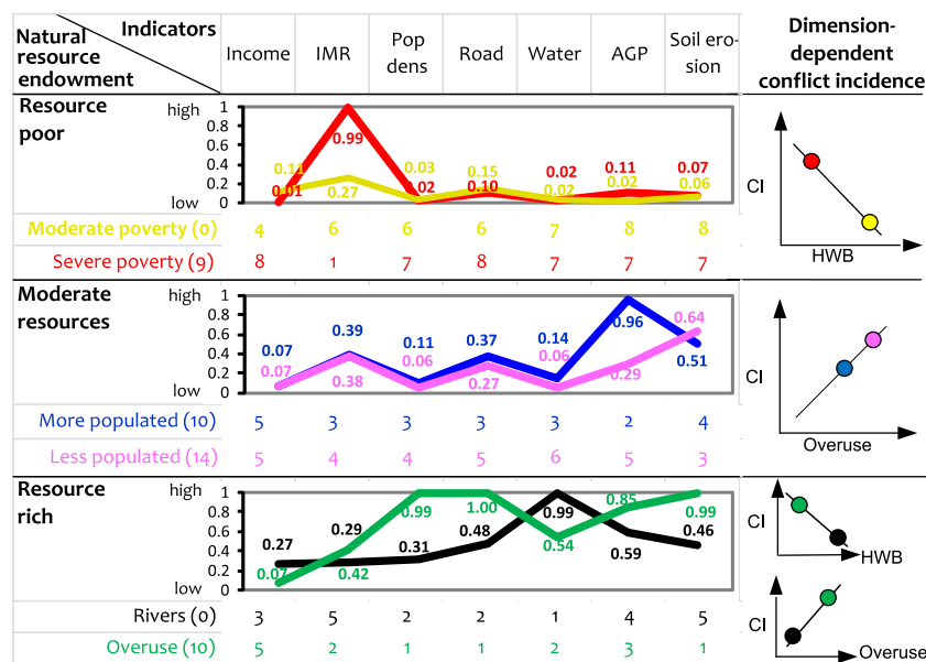
Fig. 4 Left: Vulnerability profiles of the six clusters prevalent in LMICs grouped based on poor, moderate or rich natural resource endowment, ranks of indicator values across all eight clusters (1: highest), and number of conflicts in parentheses. The indicator values are min-max normalized between 0 and 1. The reading of the indicator ranges is from “low” (0), to “high” (1), as opposed to from “adverse” to “favorable”. Column header abbreviations for indicators: Income: Average per capita income; IMR: Infant mortality rate, Pop dens: Population density, Road: Infrastructure density; Water: Renewable water resource; AGP: Agropotential; Soil erosion: Soil erosion (through water erosion). Right: Schematic diagrams of conflict incidence as a function of the dimensions of natural resource endowment, HWB, and overuse. CI means conflict incidence; Human well-being (HWB) is a function of average per capita income and IMR; Overuse is a function of soil erosion and population density. For each group of similar natural resource endowment the circles with colors corresponding to the clusters colors show how the conflict incidence (y axis) relates to different degrees of HWB or overuse (x axis). The black diagonal lines show the direction of change in conflict proneness when changing the independent variables on, and the distances between circles approximate the differences.
